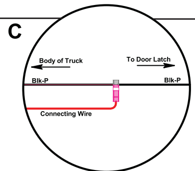
Front Door Panel (Passenger Side)
