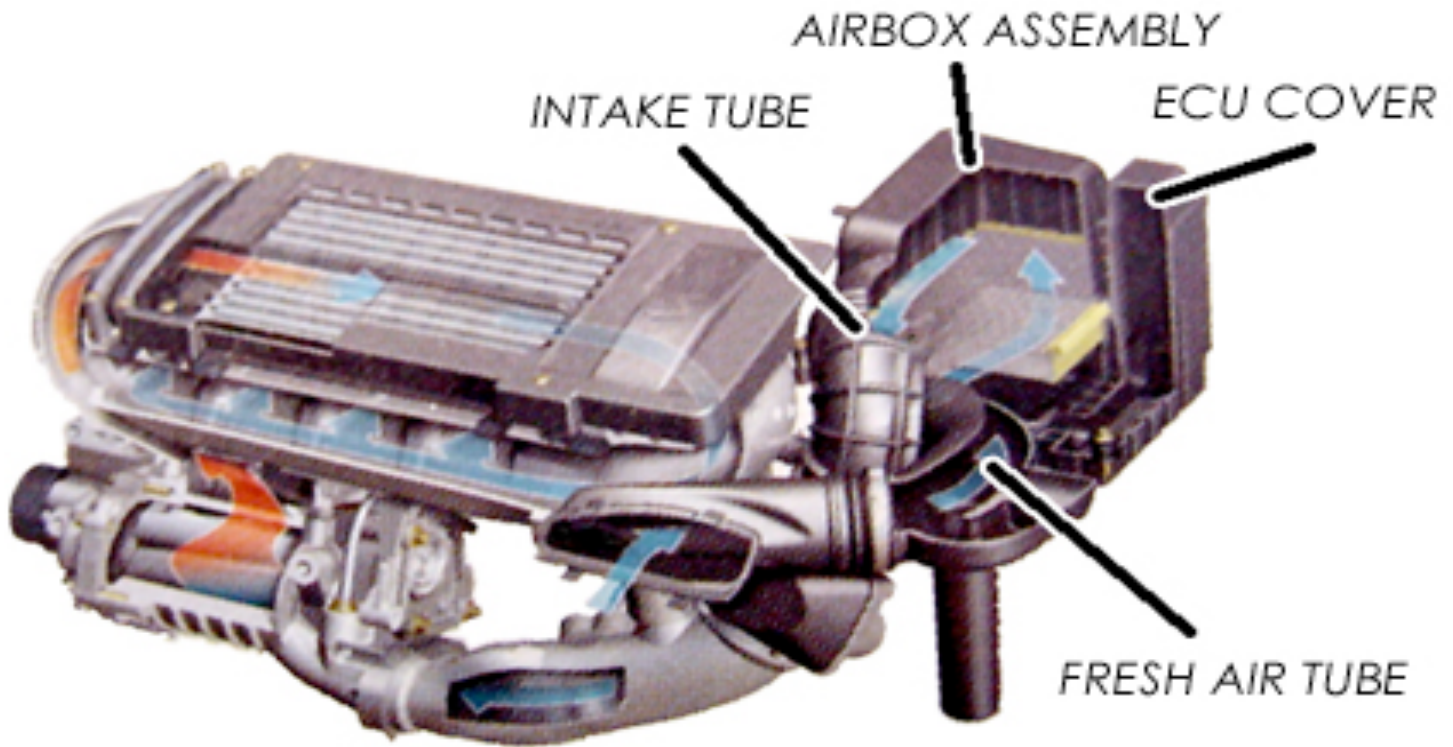
OEM SETUP
