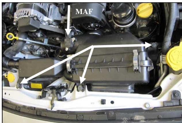
2. Disconnect the Mass Air Flow sensor, or MAF, in the airbox. Remove the three 6mm bolts securing the airbox assembly and remove it from the vehicle.
