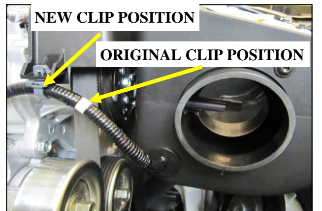
9. Route the MAF harness into the Airbox and reconnect the sensor inside. Seal off the access port with the Grommet from step 9. Relocate the plastic clip on the wire harness 1 1/4" back to take up any slack that might allow contact with the accessory belt.
