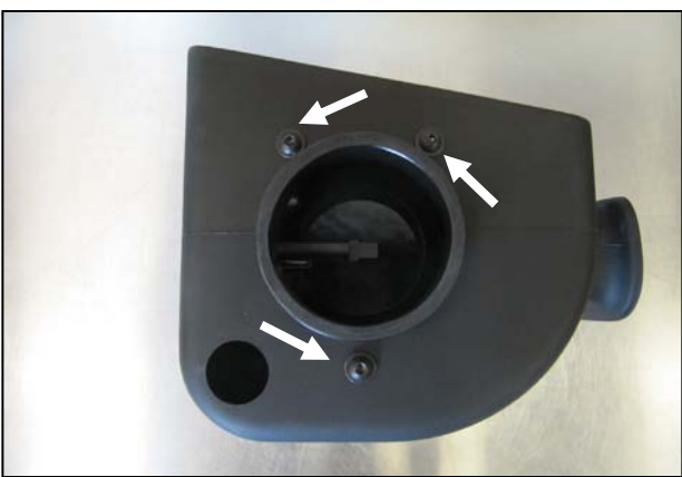
4. Install the Filter Adapter into the Cold Air Box as shown using the 1/4-20 Button Head Screws and 1/4" Flat Washers .
