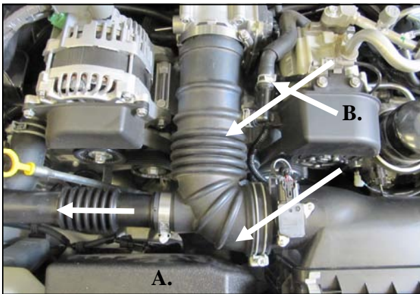
1. Disconnect The Negative Battery Terminal! Loosen the clamps on the throttle body and the airbox outlet. A. Loosen the resonator tube clamp and disconnect it from the intake. B. Compress the spring clamp on the crank case breather line and disconnect it. Remove the intake tube from the vehicle.
