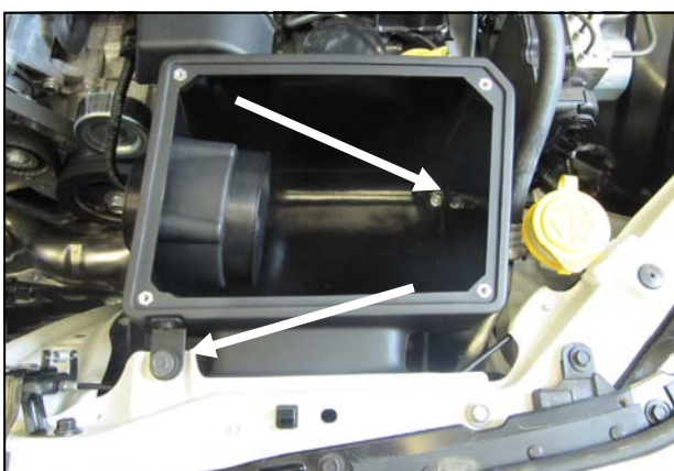
7. Slide the CAB Mount stud through the hole in the Airbox bottom and secure it using the M6 Flange Nut and a 1/4" Flat washer. Reuse one 6mm airbox bolt from step 3 to join the Airbox Bracket to the core support.
