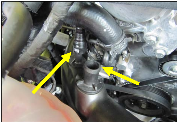
6. Disconnect the PCV and turbo bypass lines from the intake tube and remove the tube from the vehicle.
