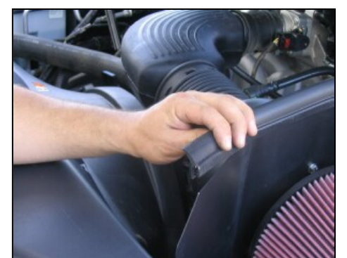
12. Install the supplied weather strip on the top edge of the Airaid Cool Air Dam. Note: The weather strip is pre cut to the proper length. Start from one end and work your way around to the other end to insure even placement.
