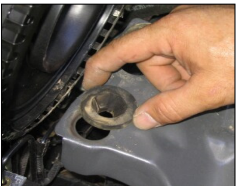
6. Remove the two factory grommets from the body and discard.
