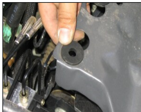
7. Install the supplied rubber grommets in place of the factory grommets previously removed.
