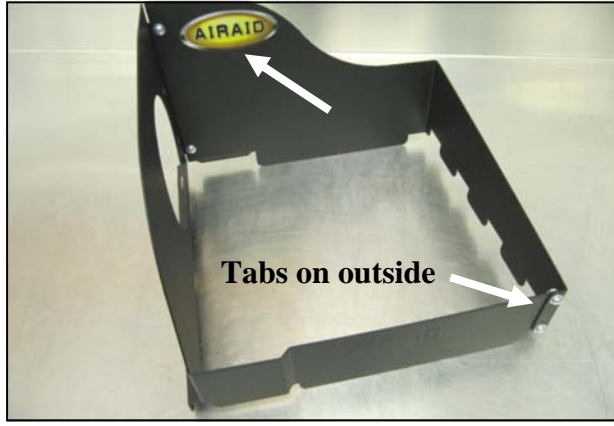
5. Assemble the Front and Rear Panels as shown with the tabs on the outside of the assembly. Use the four 6-32 Phillips Head Screws, #6 Flat Washers, and #6 Kep Nuts to secure the assembly. Apply the Airaid Decal on the completed Panel assembly as shown.
