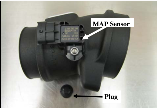
8. Transfer the MAP Sensor into the Airaid intake tube as shown. Secure the sensor using the Long 8-32 Button Head Screw and the Washer. Discard the Plug. It will not be used.
