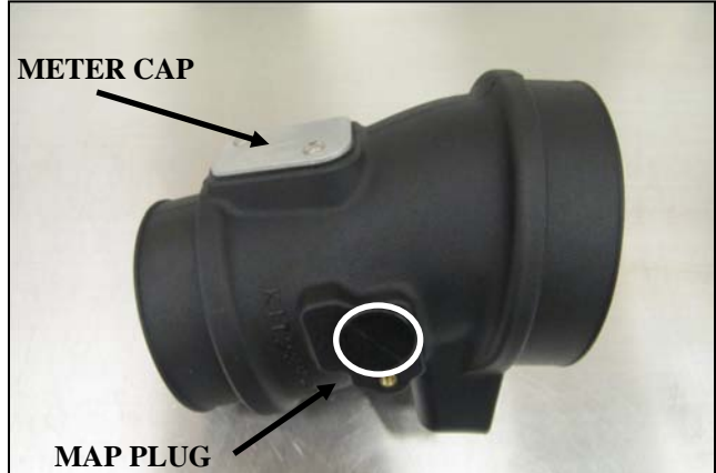
6. Depending on the sensor configuration of your factory intake system, you will use one of the two sensor receptacles in the Airaid intake tube. There is a Mass Airflow sensor receptacle on the tube and a MAP sensor receptacle on the tube.
