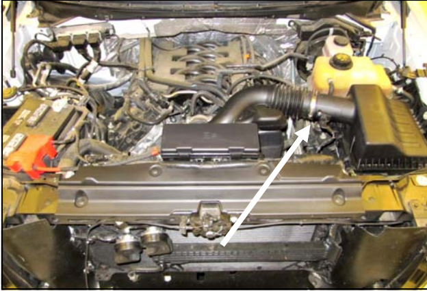
Disconnect The Negative Battery Terminal! 1. Loosen the hose clamp on the airbox side of the factory air intake tube.
