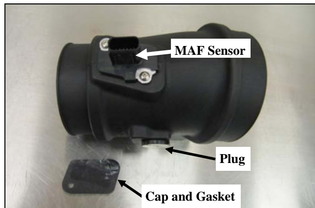
9. If your vehicles intake utilizes a Mass Airflow, or MAF sensor: Transfer the sensor into the Airaid intake tube as shown and secure using the two 1/2" Button Head Screws. Complete the Tube assembly by inserting the MAP Plug. Discard the Meter Cap and Gasket. They will not be used.
