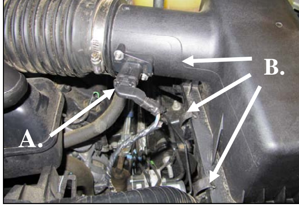
2. A. Disconnect the sensor, MAF or MAP, in the factory airbox top. B. Unfasten the Three clips on the left side of the air-box.
