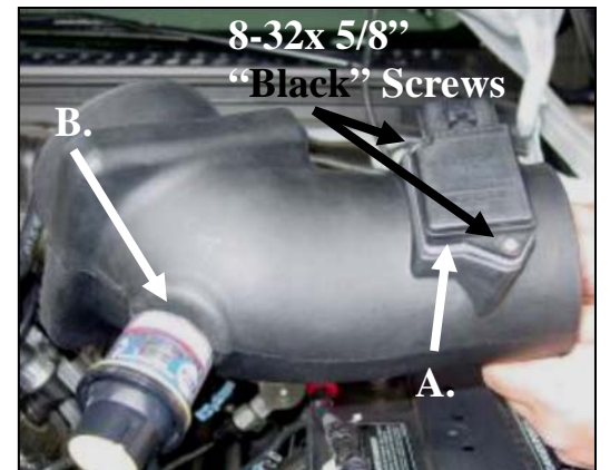
9. A.) If you have the MAF sensor shown in step #6, install the gasket (#12) and sensor using two (black) 8-32x5/8" button head bolts (#11). B.) Install the factory grommet and filter restriction gauge.
