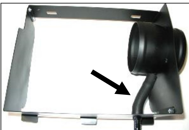
4. Install the supplied 1/2" hose on the Airaid CAD nipple. Assemble Airaid CAD panels using supplied hardware. Install supplied 1/2" nylon union through the panel hole into the 1/2" hose.
