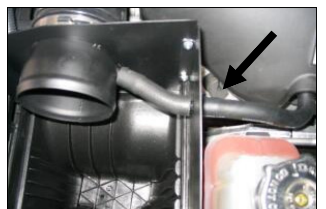
6. Connect the factory breather hose to nylon 1/2" union.
