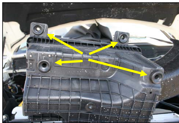
4. Remove and save four grommets from the bottom of the factory air box. They will be reused in step #5
