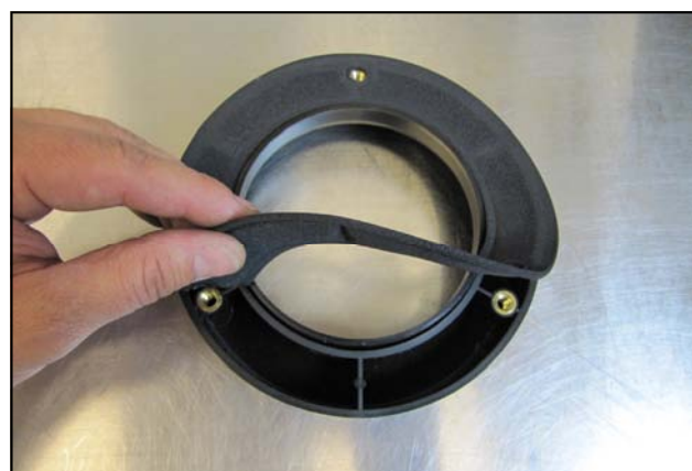
7. Prepare the Filter Adapter (#3) for installation by mating it to the Adaptor Gasket (#5) and aligning the bolt holes.
