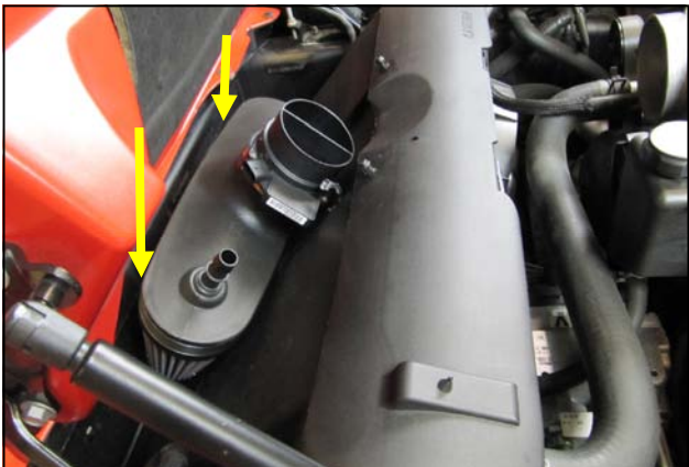
11. Install the Filter Assembly in the inner bumper area. When properly installed the Filter end cap will positively engage the grommet posts on the inner frame.
