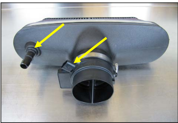
6. Transfer the Mass Air Flow meter into the Airaid Filter Assembly. Note the positioning of the air meter socket in relation to the breather coupling.
