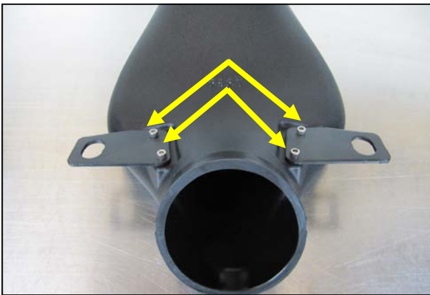
7. Install the Tube Brackets onto the Intake Tube as shown using the 8-32 Socket Head Screws (#9)
