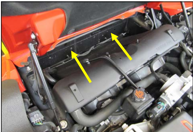
10. Inspect the inner bumper area and verify that none of the air box mounting grommets were retained during disassembly.
