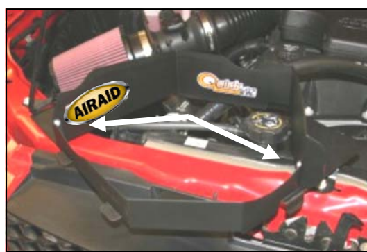
5. Assemble the Quick Fit panels (#2&#3) using the four 6-32x5/16" screws (#5), #6 washers (#7), and nuts (#6). Apply the Airaid Foil Decal onto the Panel as shown.
