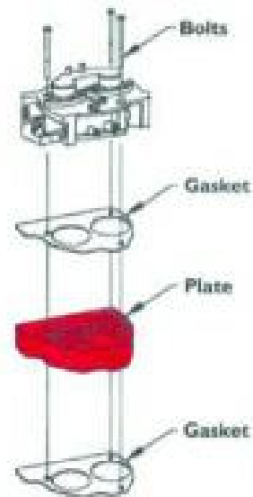
Throttle Body Showing Bolts, Gaskets, and Plate
