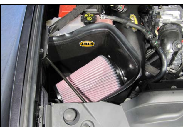
17. Install the Airaid Premium Filter onto the Intake Tube inside of the Cold Air Box. Install the Weather Strip onto the top edge of the Cold Air Box with the contour rolling away from the filter. Reinstall the fender trim and brace.
