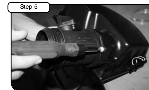
Remove MAF sensor using T30 torx bit.
