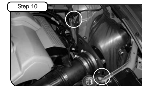
Tighten housing using bolts from step 4 and 8. Tighten all clamps using 5/16" nut driver.
