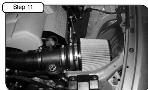
Install air filter and tighten using 5/16" nut driver. Re-connect MAF sensor harness.
