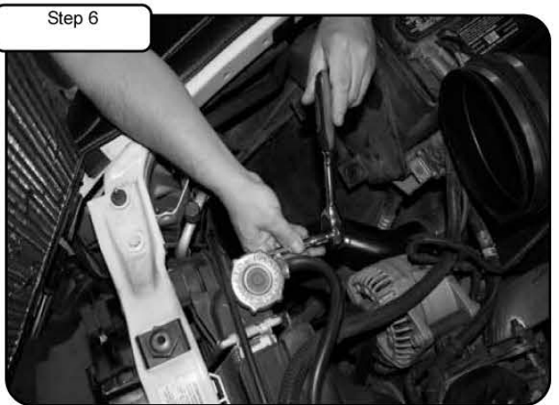
Step 6 With 10mm socket and extension loosen the two bolts holding in radiator on back of upper radiator support.
