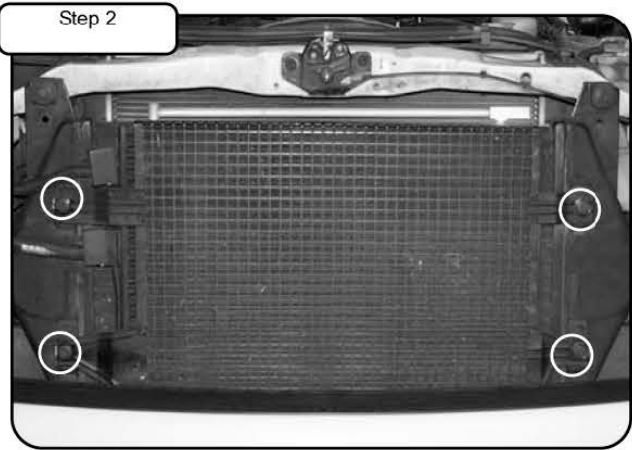
Step 2 Remove plastic A/C line protector on passenger side. With 13mm socket or wrench loosen the 4 bolts holding in A/C condenser.
