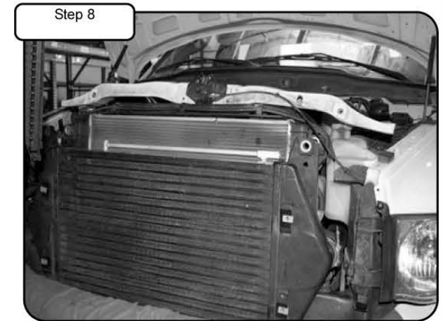
Step 8 Remove the upper radiator support and set aside on top of fan shroud. Loosen clamps on intercooler tubes using 7/16" deep socket. Now remove stock intercooler and factory couplers/clamps out of vehicle. Turn over to page 2 →
