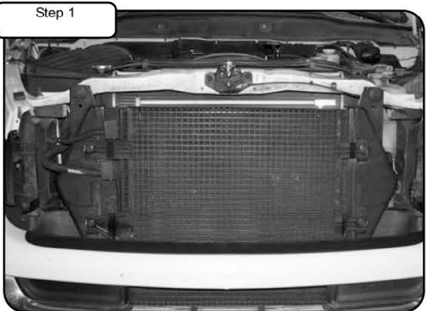
Step 1 Stock Intercooler. NOTE: Disconnect battery before install. Remove stock air box or intake system from vehicle for easier installation.
