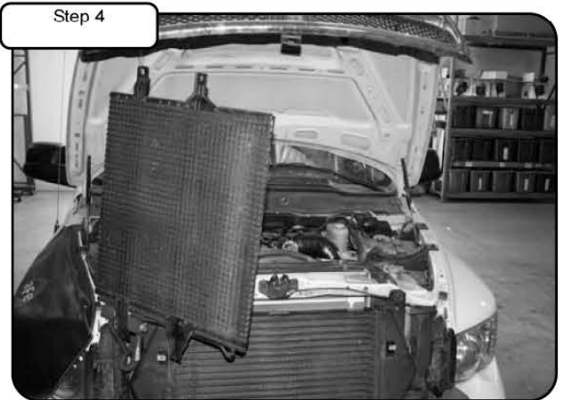
Step 4 With A/C condenser turned 90 degrees, secure to the vehicles lifted hood using steel wire.
