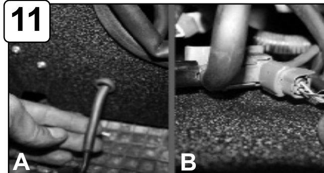
11 A) Install grommet to hole in housing. Run vacuum line through grommet and reattach to vehicle. B) Re-connect sensor harness.
