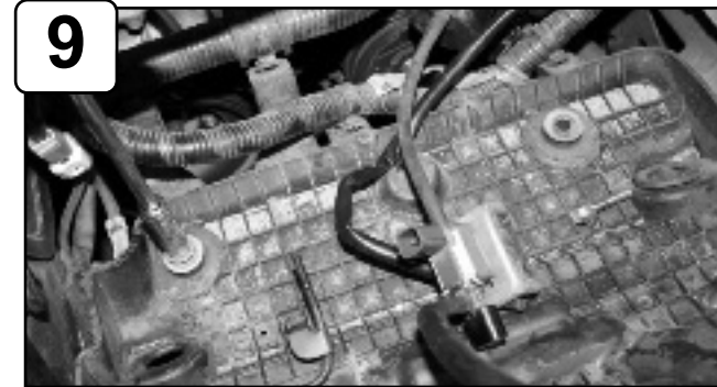
Loosen the 2 OE screws holding in air box bracket. Save for later install.
