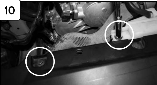
10 With 10mm socket or wrench loosen the 2 bolts on radiator reservoir and support.
