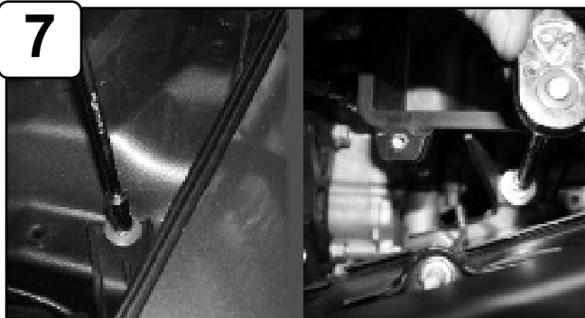
With 10mm socket or wrench loosen both bolts on stock bottom air box and remove.
