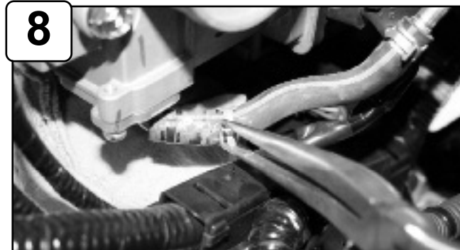
Remove crank case line attached with throttle body coolant line. Have a shop towel or rag handy to catch any leaking coolant. Use pliers to remove both lines. Save small clamps for later install. Caution: Coolant may leak from line when removing!
