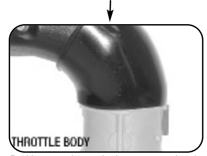
THROTTLE BODY Position coupler and clamps over throttle body (3.5" x 4.0") (clamps removed for clarification). The smaller (3.5") end of the coupler goes over the throttle body. The (4") end of the coupler goes around the intake tube.
