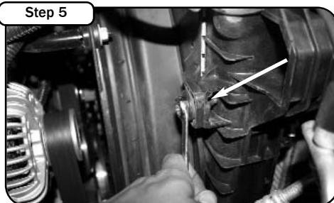
Loosen and remove the 13mm radiator bolt. Set aside for later use.
