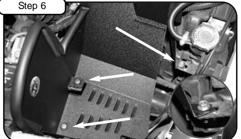
With 3/8" screws/nuts and washers provided install bottom of housing to factory position. Tighten using 9/16" wrench or socket. Use M6 screw/nut and washer and tighten housing to bracket "D" from Step 4 and tighten.
