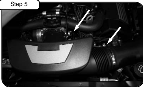
With 1/4" nut driver loosen the OE intake tube from throttle body and airbox. Remove intake tube out of vehicle.
