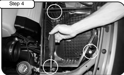
Step 4 Loosen the 3 bolts holding in bottom half of air box. Take air box out of vehicle.
