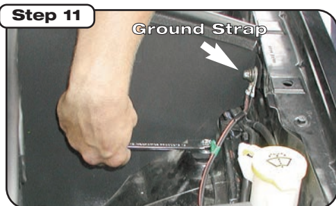
Use ground strap hardware for inner fender for mounting.
