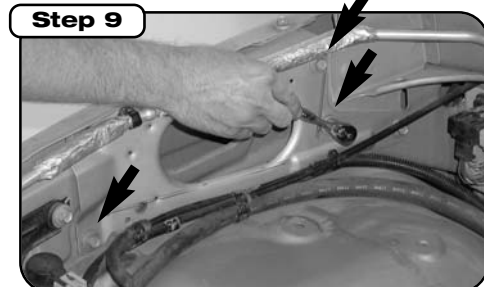
Remove three inner-fender bolts (13mm socket or wrench) for attachment of filter housing.
