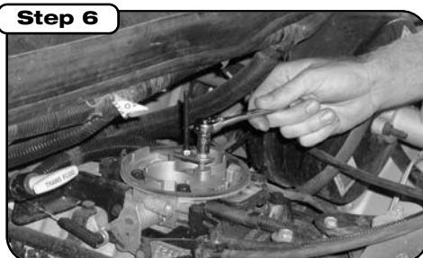
Install throttle body cap hold down bracket assembly.
