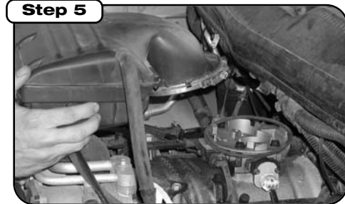
Once clamp is loose, pull up and out. Reuse existing gasket.
