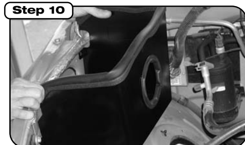
Install large housing trim seal to top of housing and small trim seal to tube inlet. Attach filter housing to inner fender-well with the three specified bolts.
