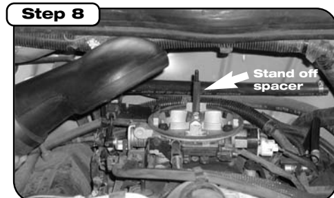
Install throttle cap stand off spacer (arrow) and cap. Reuse original throttle body gasket.
