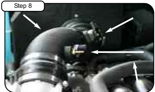
Remove MAF sensor from OE air box using phillips screwdriver. Re-install to new aFe tube with hardware provided (make sure gasket and nylon spacers are between tube and sensor) using flat head screwdriver. Install brass hose fitting.
