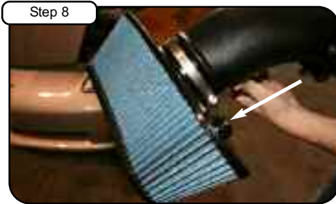
Install air filter and tighten with 5/16" nut driver. Place 3/4" cap through hole on filter.
