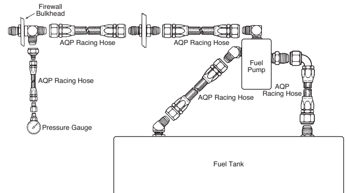
Typical Fuel System Schematic
