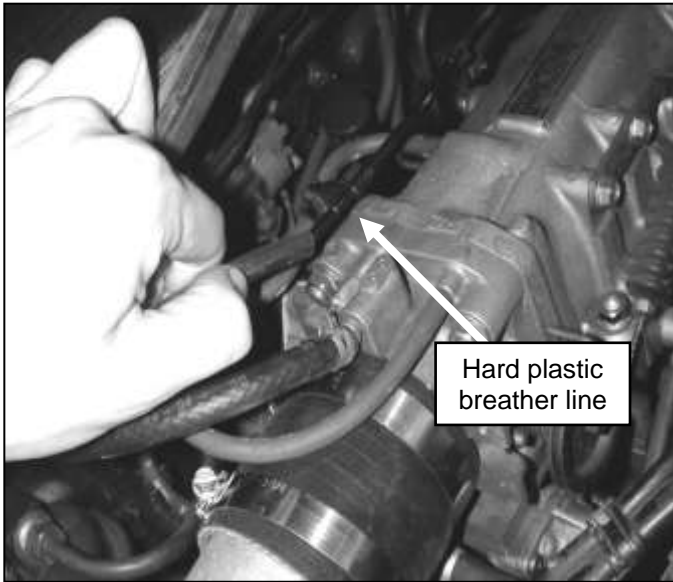
h. Remove the original 5/32" breather line that was between the stock intake pipe and the hard plastic breather line. Install the supplied longer 5/32" vacuum hose and attach it to the nipple on the backside of the intake pipe.
