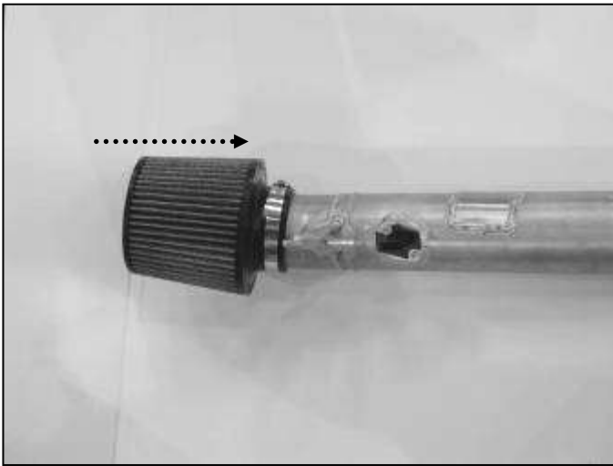
l. Attach the air filter element to the end of the inlet pipe. Secure with hose clamp.
