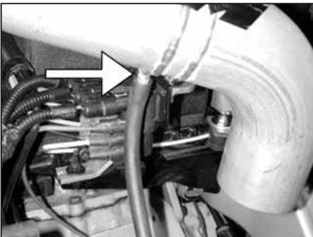
m. Attach vacuum hose to the breather nipple on the underside of the pipe and secure with hose clamp.
