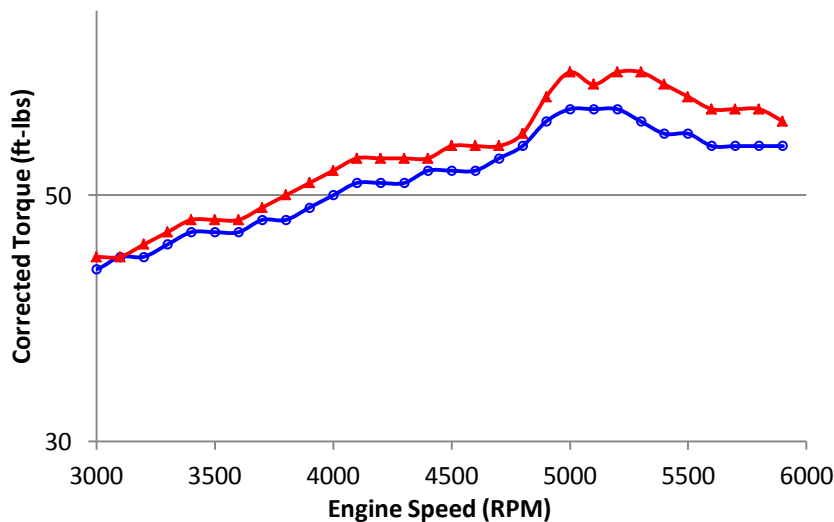
Corrected Torque (ft-lbs) vs. Engine Speed (RPM) 2014 Chevrolet Spark 1.2L L4
