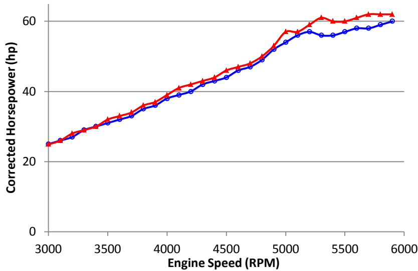
Corrected Horsepower (hp) vs. Engine Speed (RPM) 2014 Chevrolet Spark 1.2L L4
