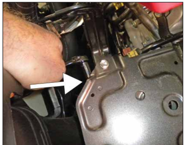
v. Remove the 10mm bolt securing the intake duct.
