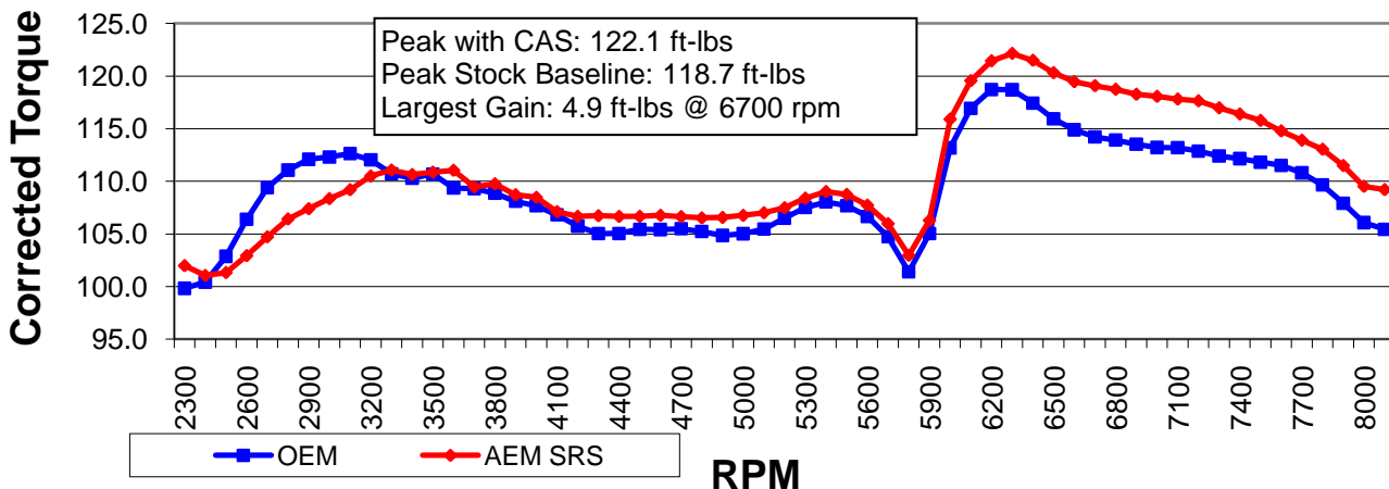
Corrected Torque (ft-lbs) vs. Engine Speed (RPM)
