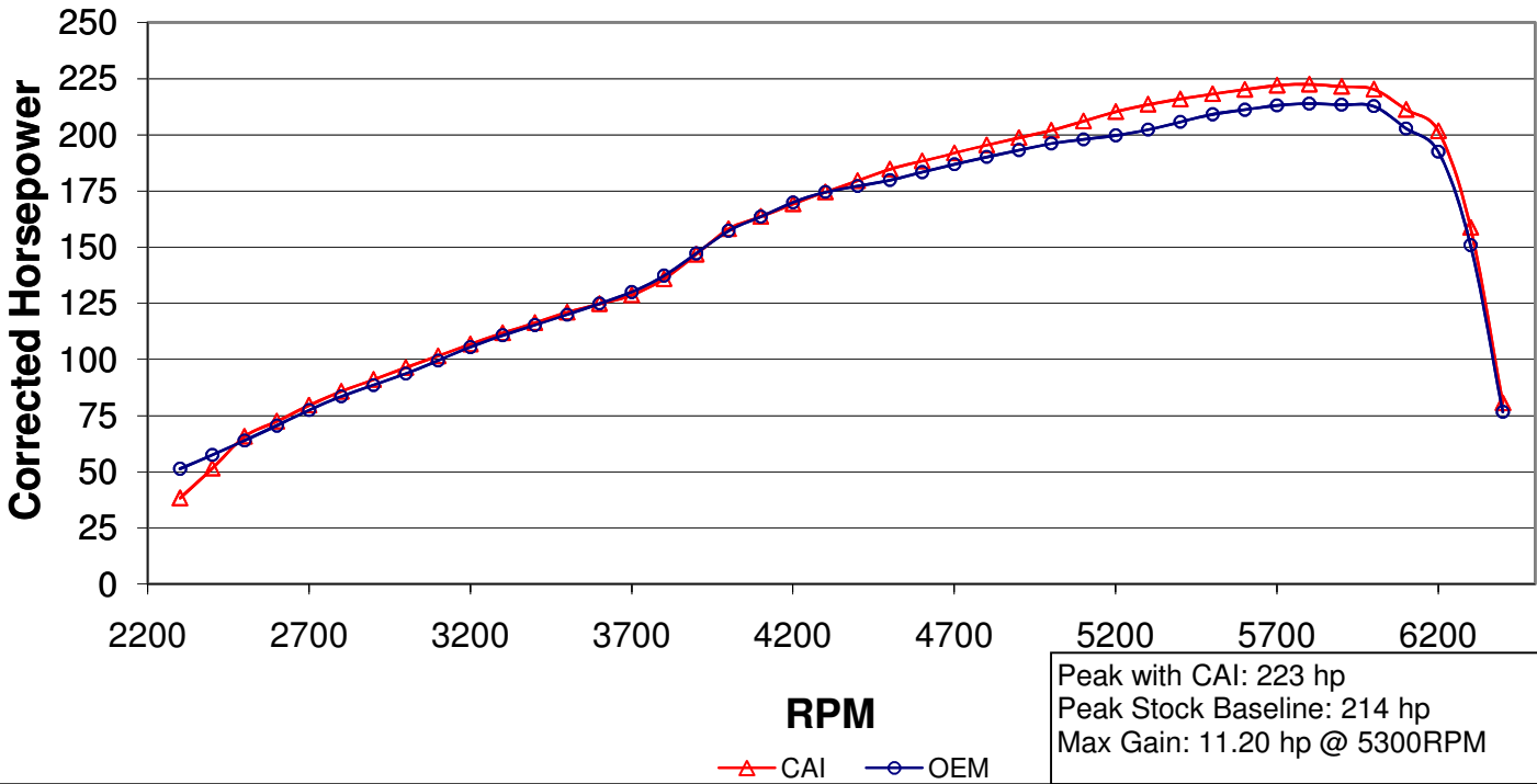
Corrected Power (hp) vs. Engine Speed (RPM)
