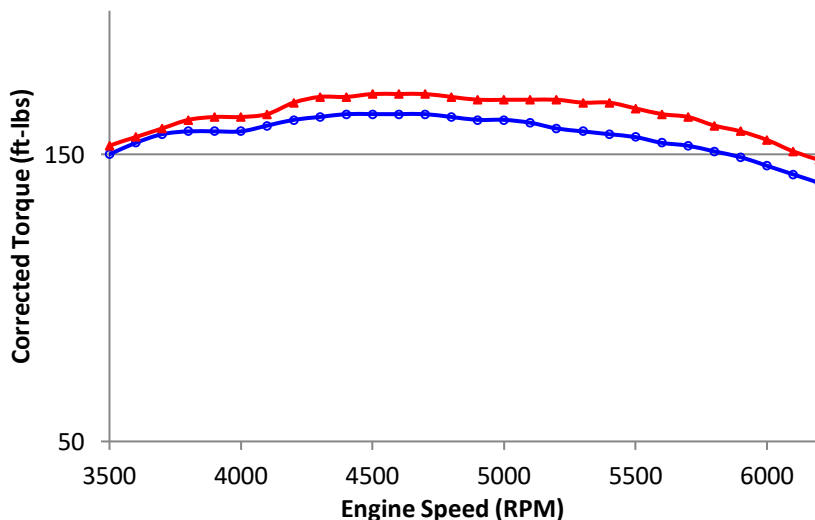
Corrected Torque (ft-lbs) vs. Engine Speed (RPM) 2017 Hyundai Elantra 1.6L Turbo
