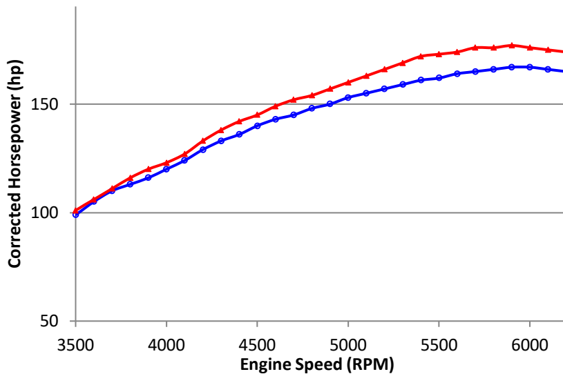
Corrected Horsepower (hp) vs. Engine Speed (RPM) 2017 Hyundai Elantra 1.6L Turbo
