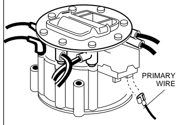
Fig. 3 Disabled GM HEI Ignition System
