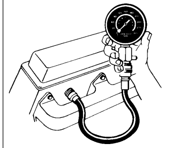
Fig. 4 Installation of Compression Gauge
