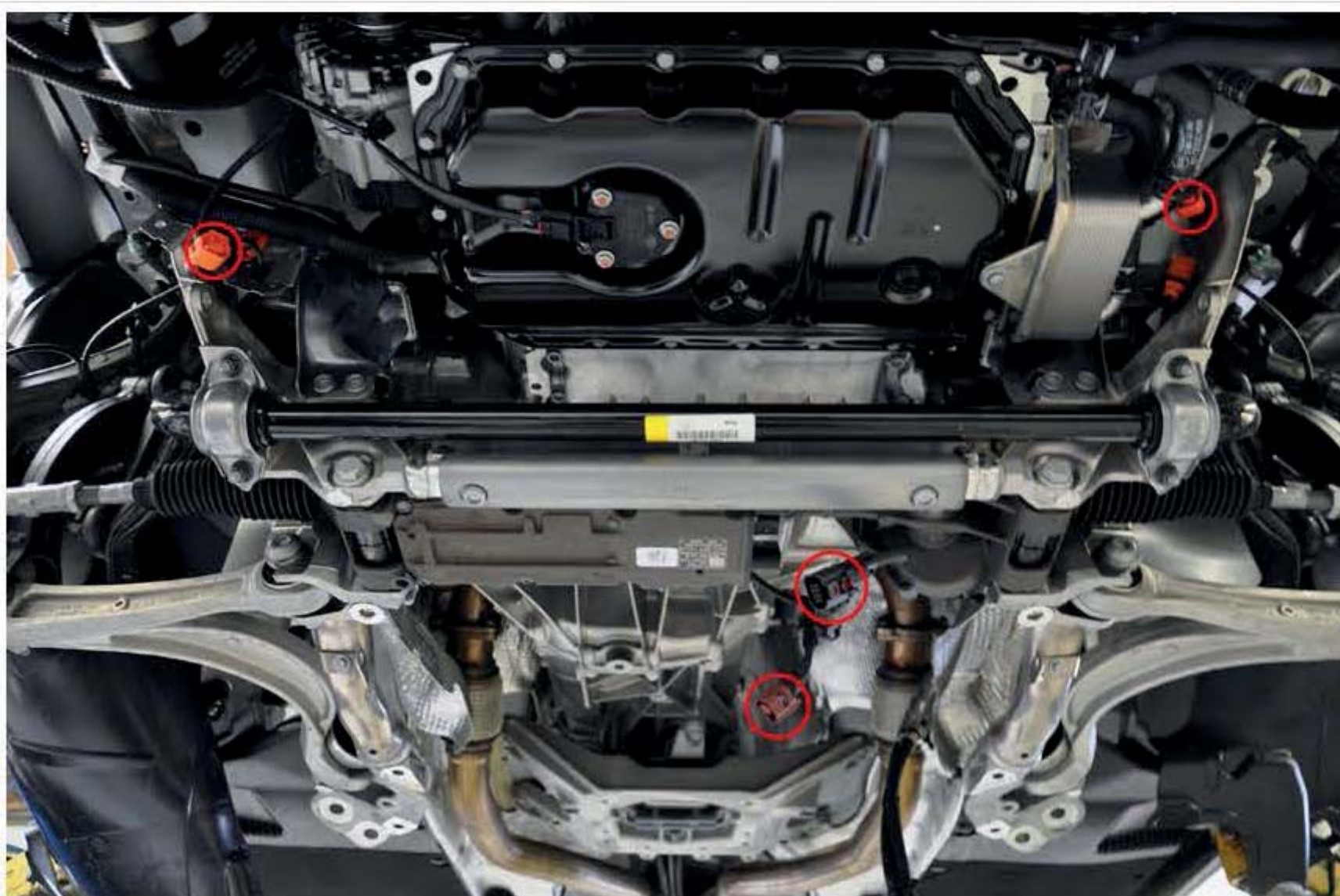
Step 6 – Disconnect the connectors circled in red, and remove the nut/bracket holding the N145 harness to the subframe.
