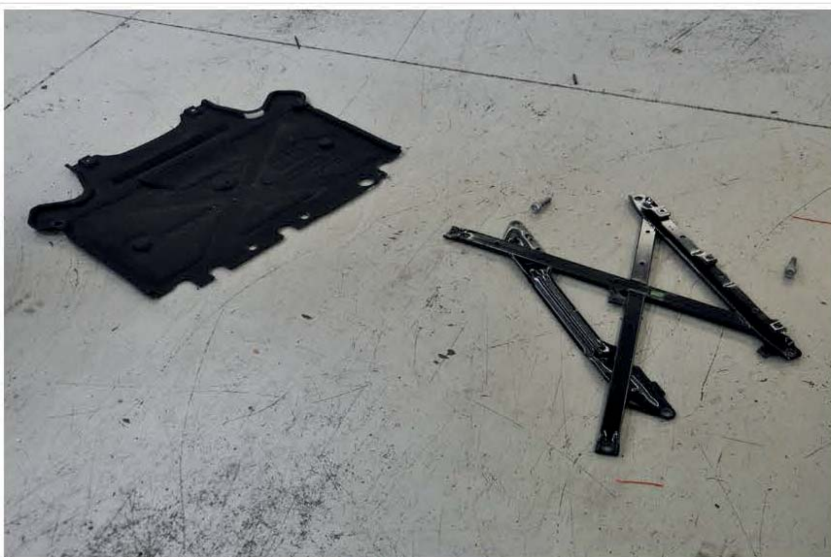
Step 5 – From here, you can either follow the factory procedure and replace one side at a time, or opt to lower the entire subframe and replace both mounts at the same time. Lowering the entire subframe requires the removal of more hardware, but may provide for easier access to the engine mounts. Lowering the subframe is highlighted below.
